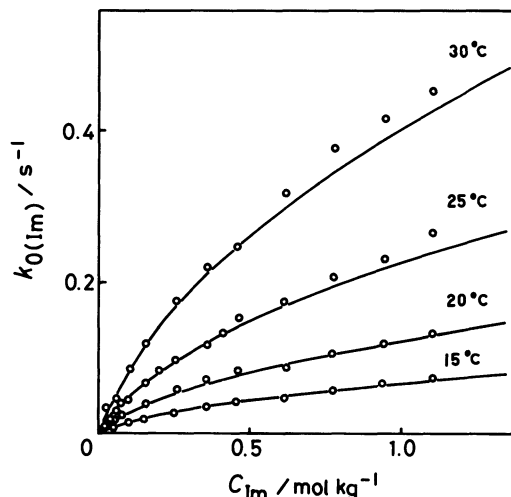
Fig. 1. Imidazole concentration dependence of first-order rate constants under atmospheric pressure at 15.0, 20.0, 25.0, and 30.0 °C. In Figs. 1—6, each point is an average of several runs. In Figs. 1, 3, 5, and 6, the solid lines were calculated by using the values obtained.
